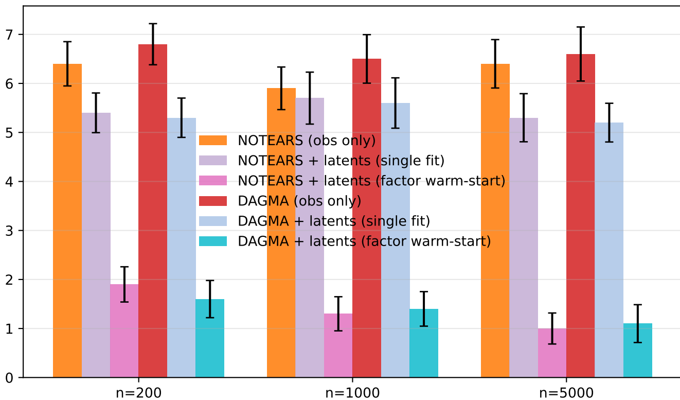
Spurious confounder-induced edges (lower is better)
